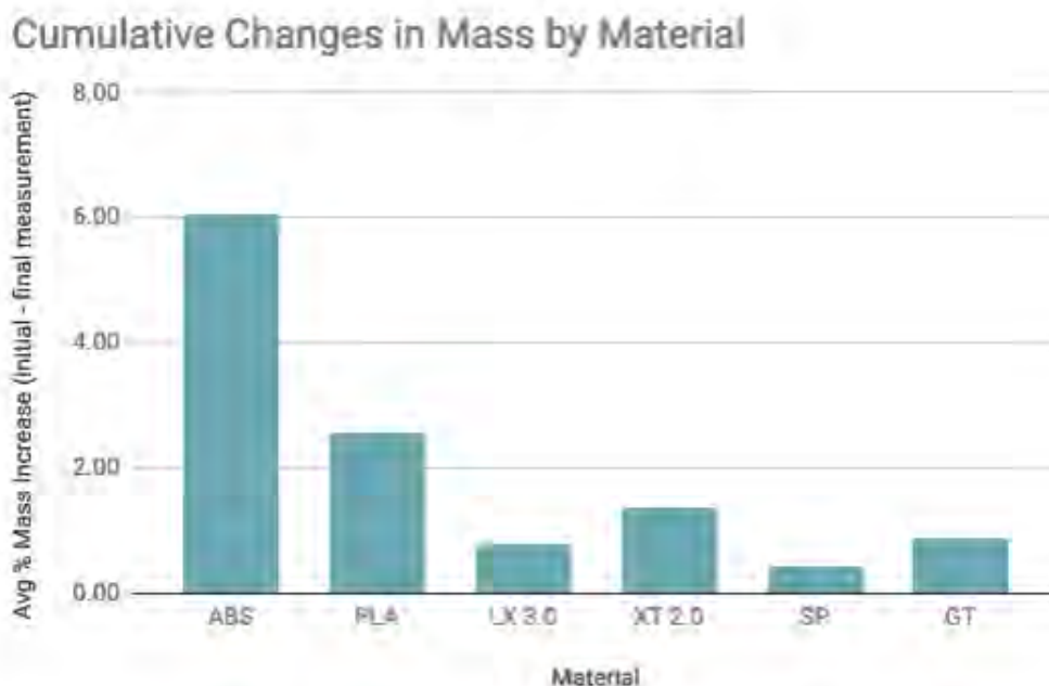
Figure 5.1: Final percent mass increases in each material (ABS, PLA, and four variants of Windform), averaged across all samples. The greater changes reflected in ABS and PLA are likely because of the lower filament density in our own prints, compared to the Winform samples given by CRP Technologies.
