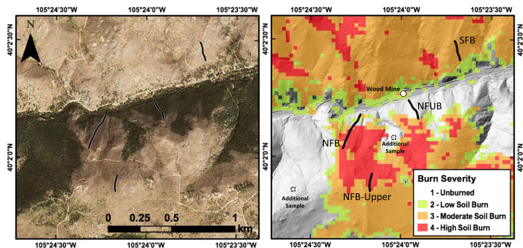
Figure 4. Burn intensity map of the study site with locations of the three soil catena transects. NFB, north-facing burned slope; SFB, south-facing burned slope; NFUB, north-facing unburned slope (control). Boxes indicate where additional reference soil cores were collected outside of the catena transects. Burn severity data based on the normalized burn ratio as part of the USGS FIREMON program (Lutes et al. , 2006). [Colour figure can be viewed at wileyonlinelibrary.com ]
