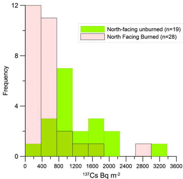
Figure 6. Histogram showing the distribution of ^{137}\text{Cs} inventories measured on the north-facing unburned and north-facing burned hillslopes. [Colour figure can be viewed at wileyonlinelibrary.com ]
