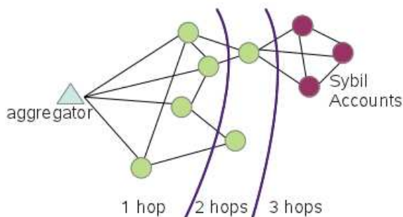
Fig. 9: Sybil accounts are often in “pockets” created by the small cut property. As a result the edges that make the small cut will be congested with votes unlike edges between legitimate users.
